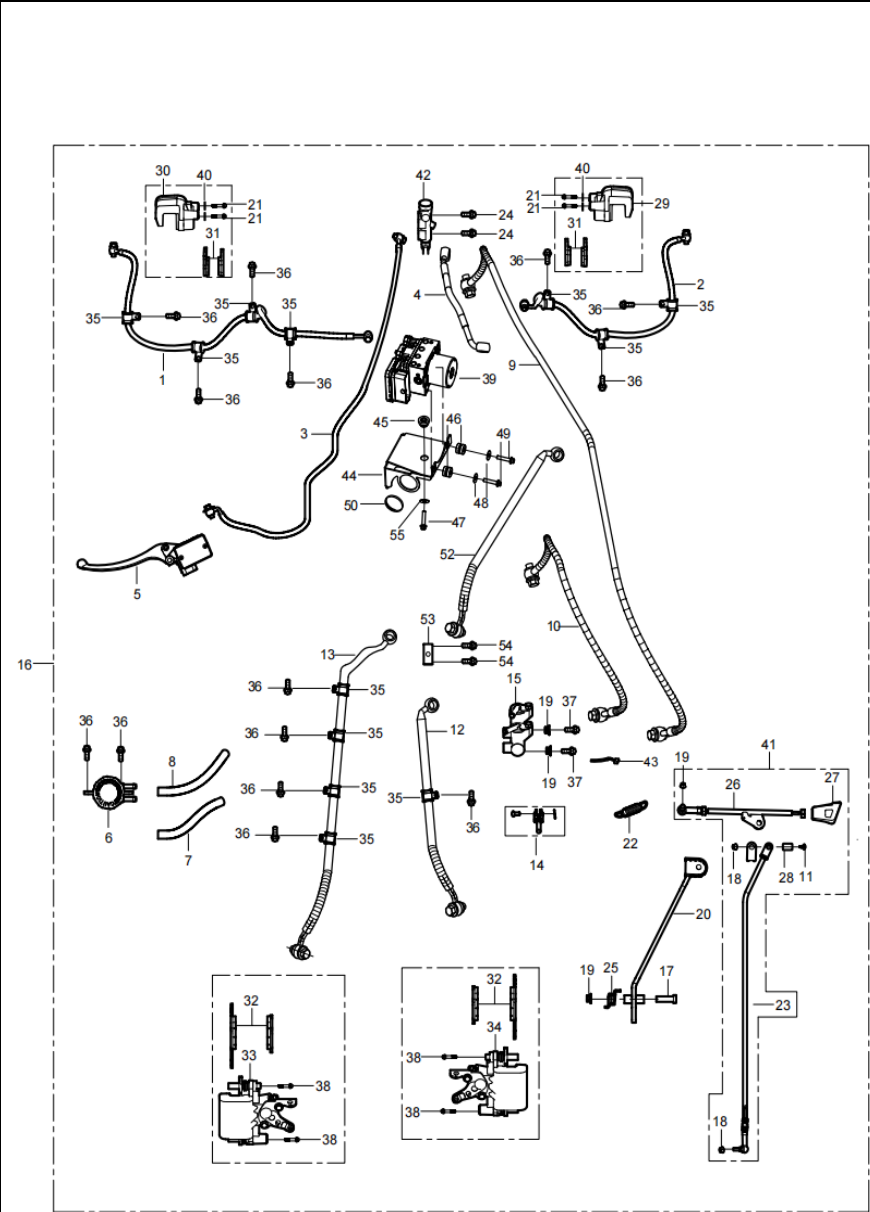
DIAGRAM 2026 BRAKING SYSTEM (ABS) F12-1
