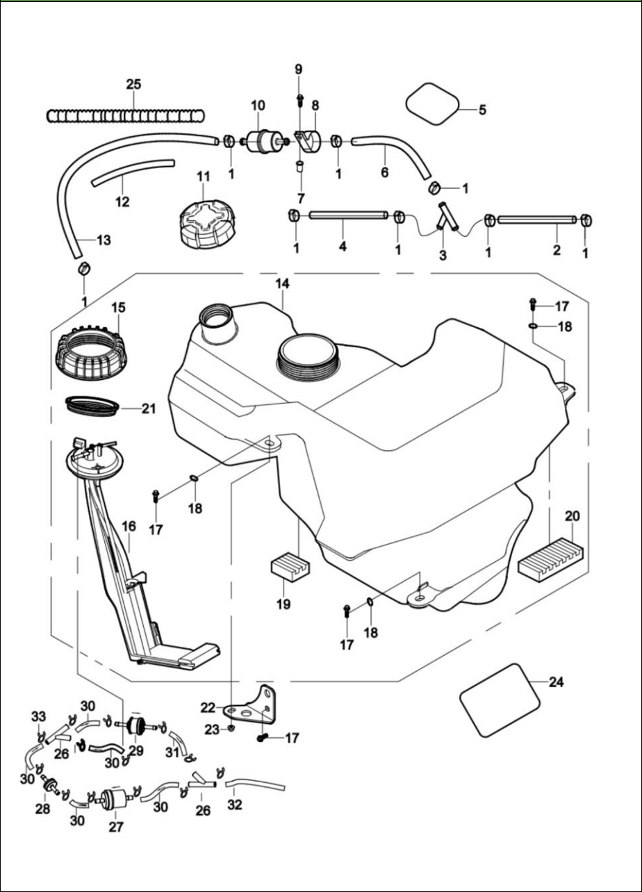
DIAGRAM 2026 FUEL SYSTEM F08
