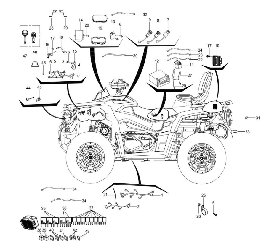
DIAGRAM 2026 ELECTRICAL PARTS F16
