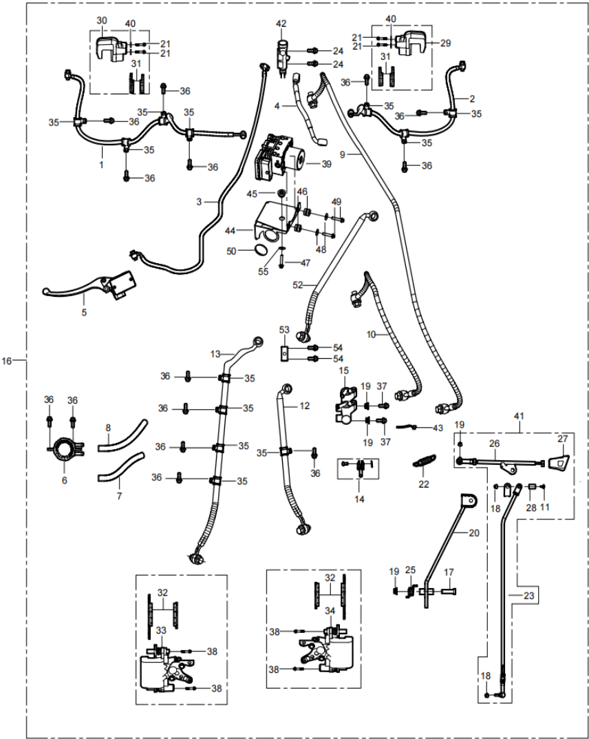
DIAGRAM 2026 BRAKING SYSTEM (ABS) F12-1
