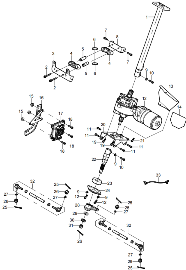
DIAGRAM 2026 STEERING SYSTEM(SEPARATED EPS) F06
