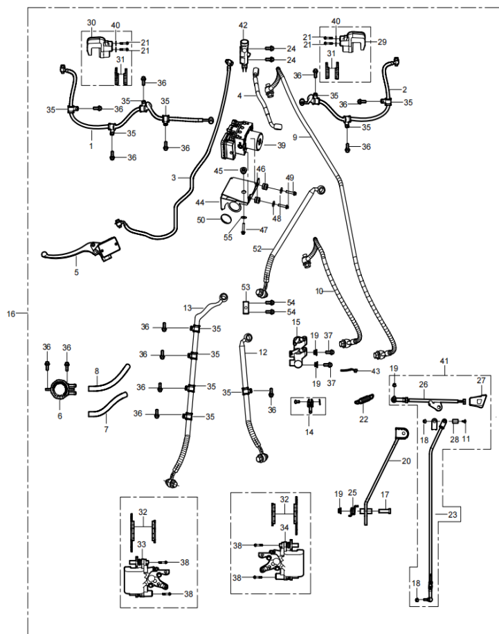
DIAGRAM 2026 BRAKING SYSTEM (ABS) F12-1
