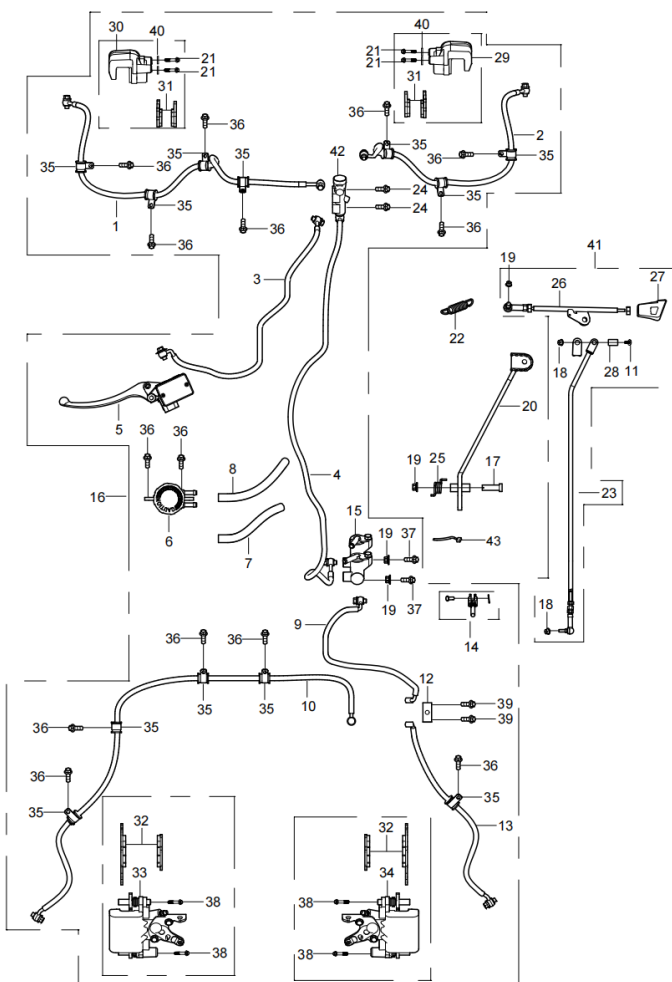
DIAGRAM 2026 BRAKING SYSTEM F12
