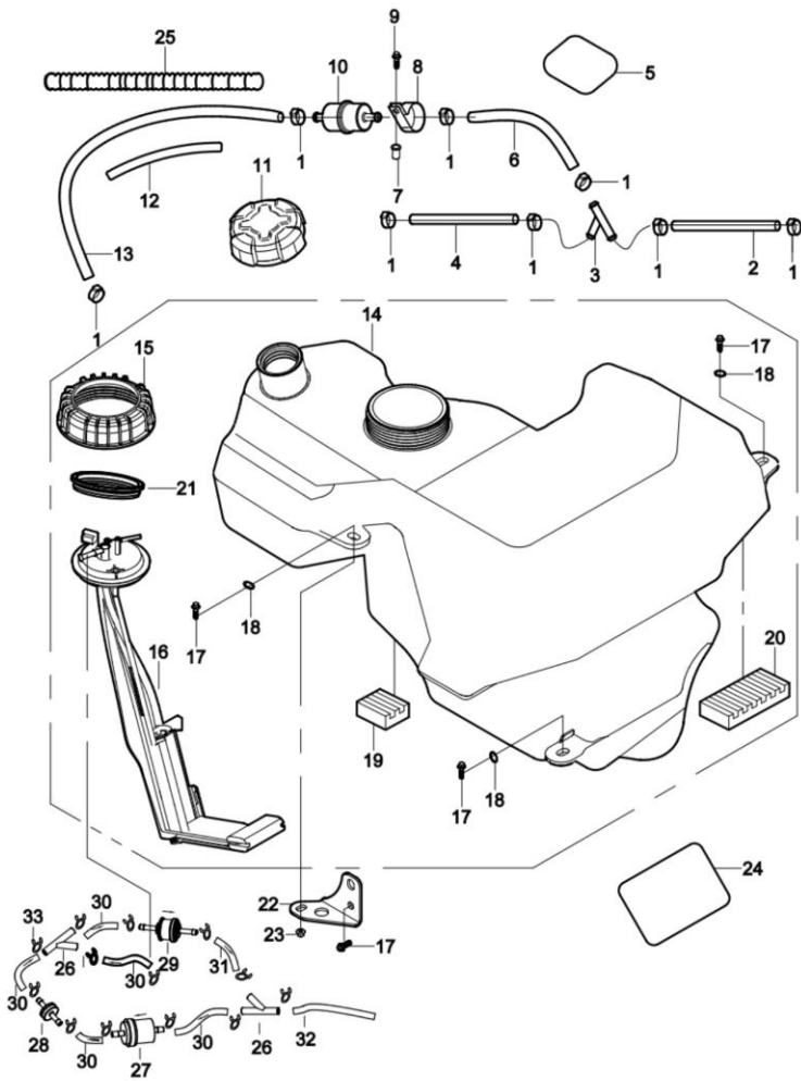
DIAGRAM 2026 FUEL SYSTEM F08
