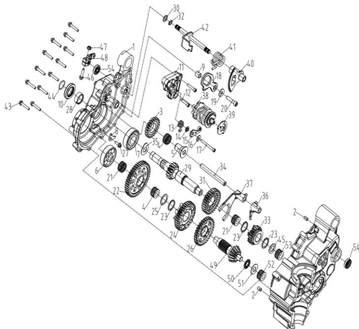
DIAGRAM 2026 GEAR BOX 1 E08
