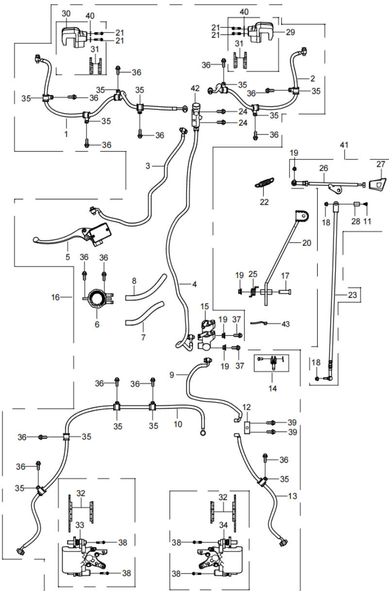
DIAGRAM 2026 BRAKING SYSTEM F12
