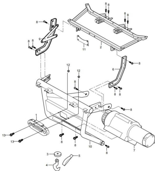
DIAGRAM 2026 FRONT WINCH ASSY (WITH FRONT BUMPER) F23
