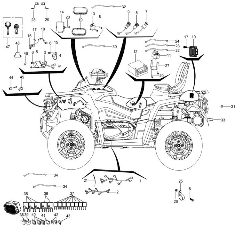
DIAGRAM 2026 ELECTRICAL PARTS F16
