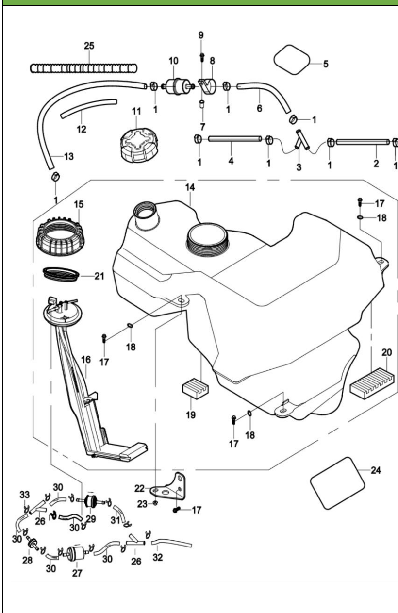
DIAGRAM 2026 FUEL SYSTEM F08
