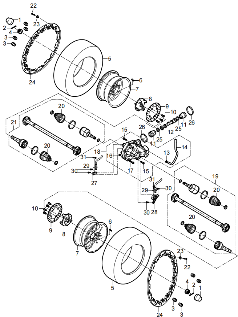
DIAGRAM 2026 FRONT DRIVE SYSTEM (ABS) F01-1
