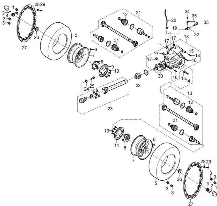
DIAGRAM 2026 REAR DRIVE SYSTEM (ABS) F02-1
