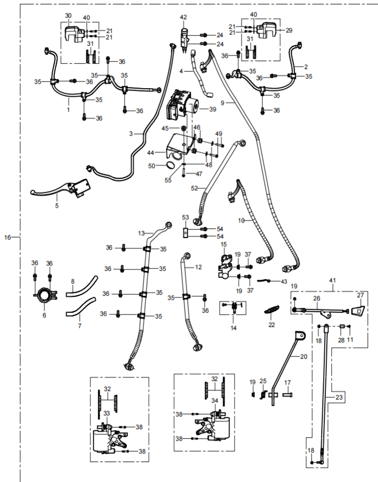
DIAGRAM 2026 BRAKING SYSTEM (ABS) F12-1
