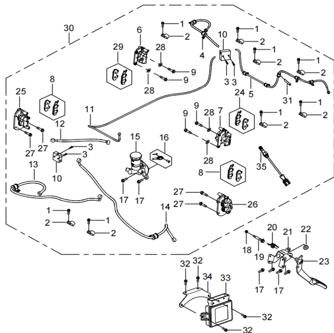
DIAGRAM 2026 BRAKING SYSTEM F16
