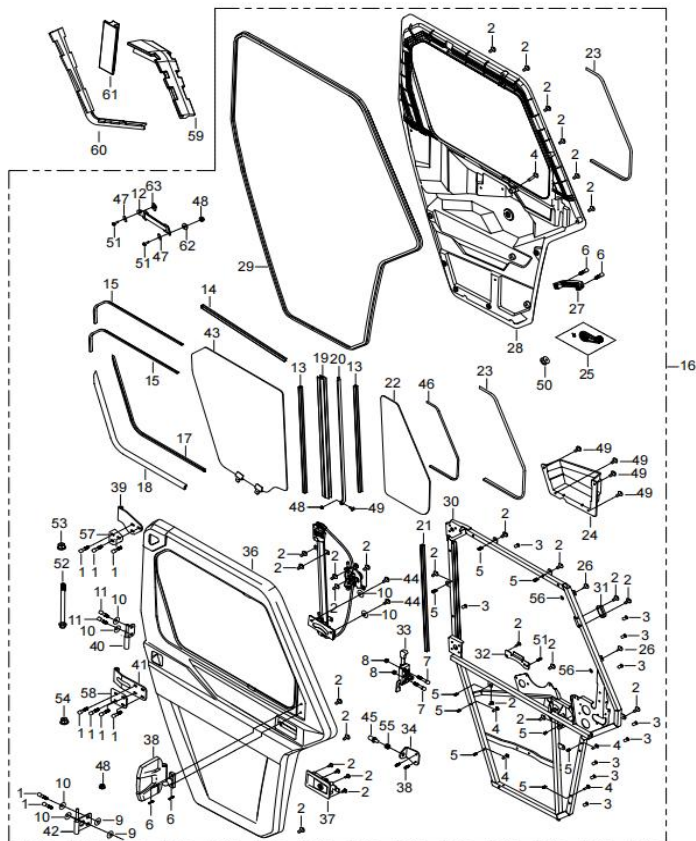
DIAGRAM 2026 FRONT DOOR PASSENGER SIDE (TWO DOOR) F25-Part 1
