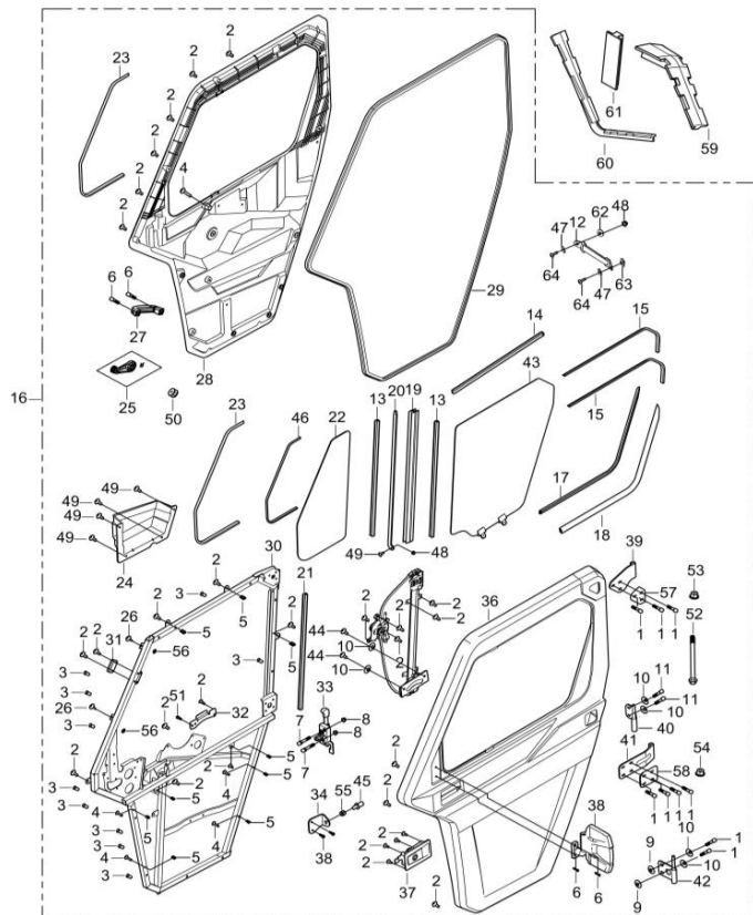
DIAGRAM 2026 FRONT DOOR DRIVER SIDE (TWO DOOR) F24-Part 1
