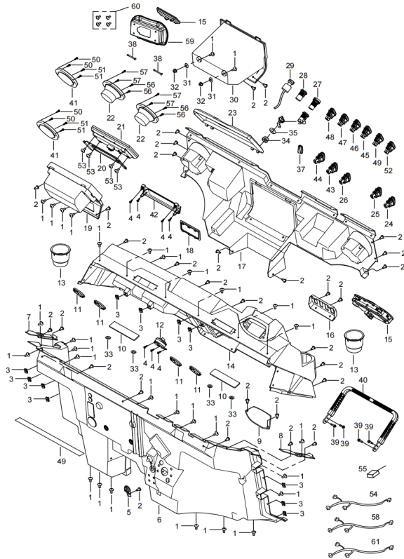
DIAGRAM 2026 DASH BOARD (WITHOUT HEATER/AC ) F17 - Part 2
