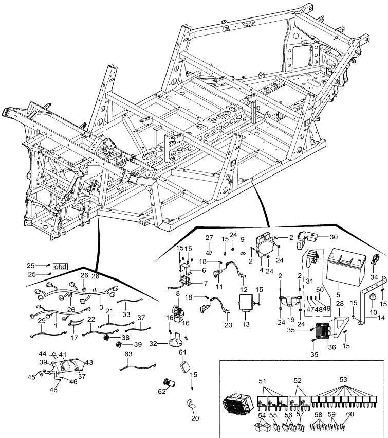
DIAGRAM 2026 ELECTRICAL COMPONENTS F22-Part 1
