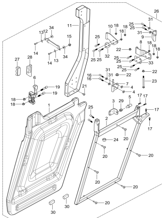
DIAGRAM 2026 FRONT DOOR PASSENGER SIDE (FOUR DOOR) F27-Part 1
