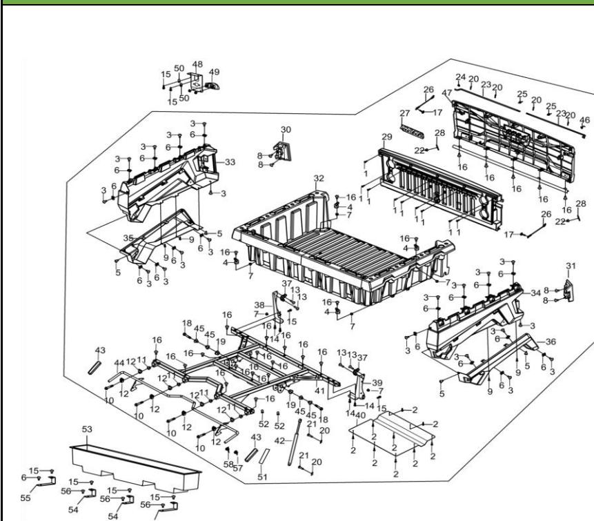
DIAGRAM 2026 CARGO BOX F23
