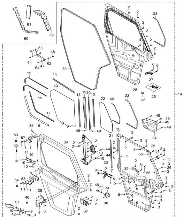
DIAGRAM 2026 FRONT DOOR PASSENGER SIDE (TWO DOOR) F29-Part 1
