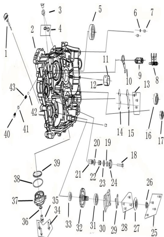
DIAGRAM 2026 LEFT CRANKCASE B
