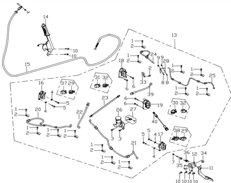
DIAGRAM 2026 BRAKING SYSTEM F18
