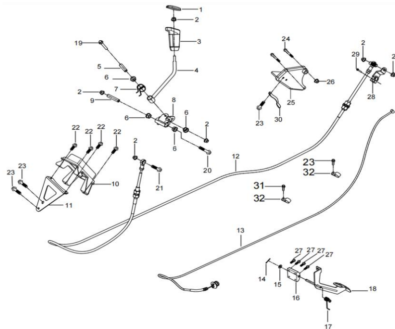
DIAGRAM 2026 SHIFT AND THROTTLE CONTROL SYSTEM F12
