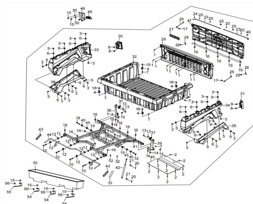
DIAGRAM 2026 CARGO BOX F23
