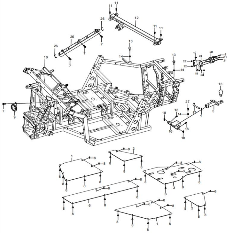
DIAGRAM 2026 FRAME (TWO DOOR) F17
