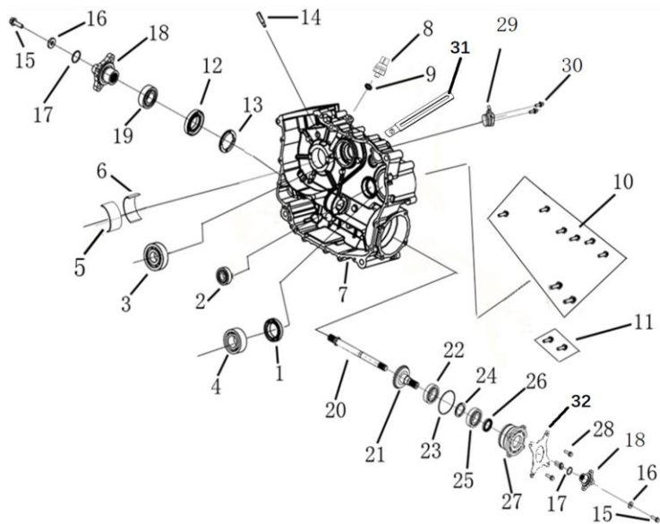
DIAGRAM 2026 RIGHT CRANKCASE
