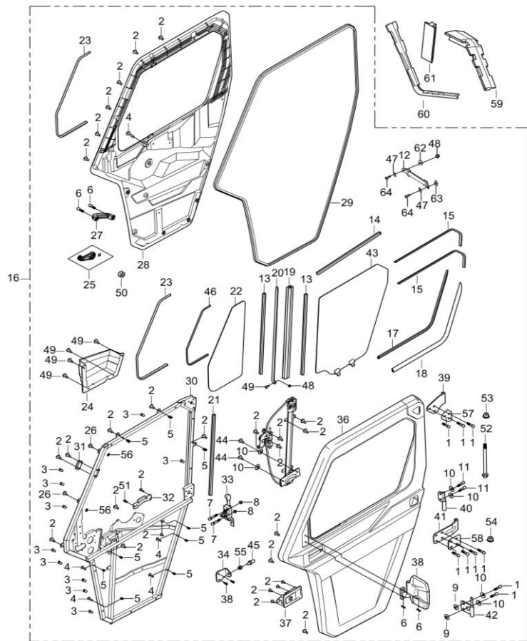
DIAGRAM 2026 FRONT DOOR DRIVER SIDE (TWO DOOR) F24-Part 2
