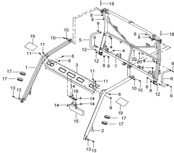
DIAGRAM 2026 ROLL BAR (TWO DOOR) F11
