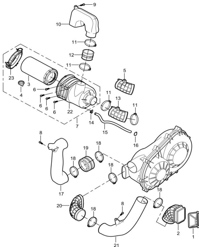
DIAGRAM 2026 AIR FILTER & CVT INLET&OUTLET SYSTEM F09
