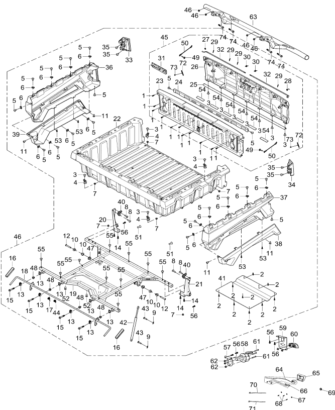
DIAGRAM 2026 CARGO BOX F21-Part 4
