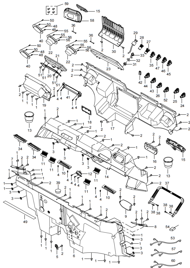
DIAGRAM 2026 DASH BOARD (WITH heater/AC ) F18 Part-1
