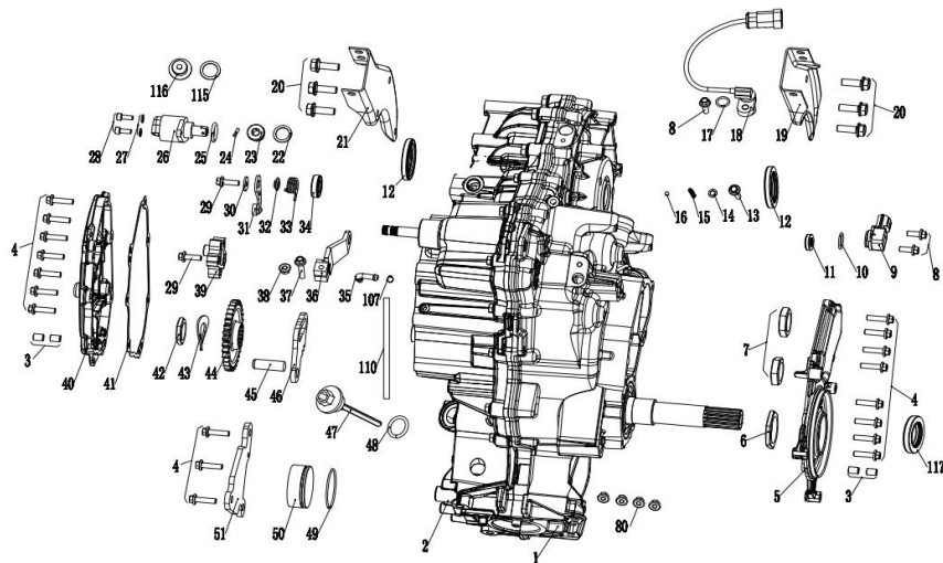
DIAGRAM 2026 TRANSMISSION E08
