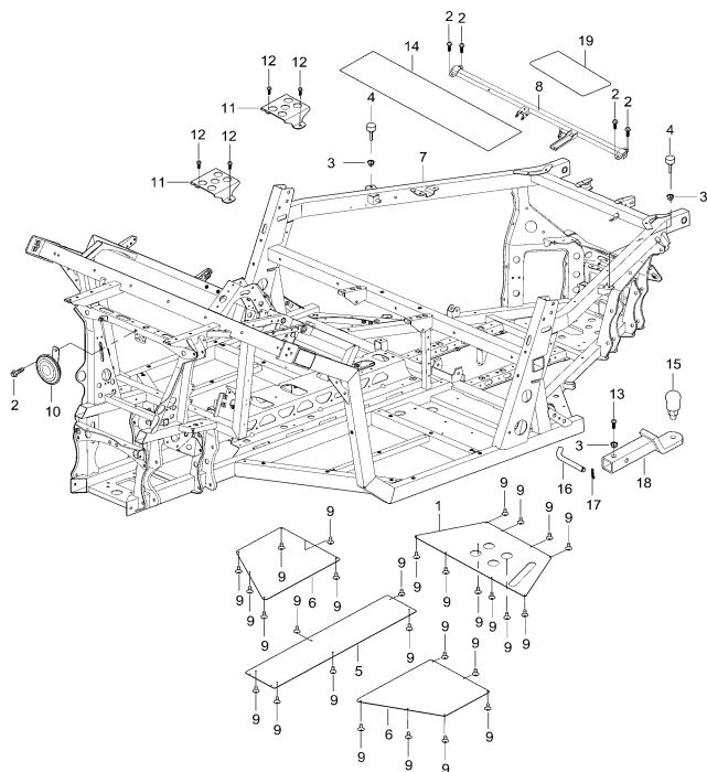
DIAGRAM 2026 FRAME (TWO DOOR) F15
