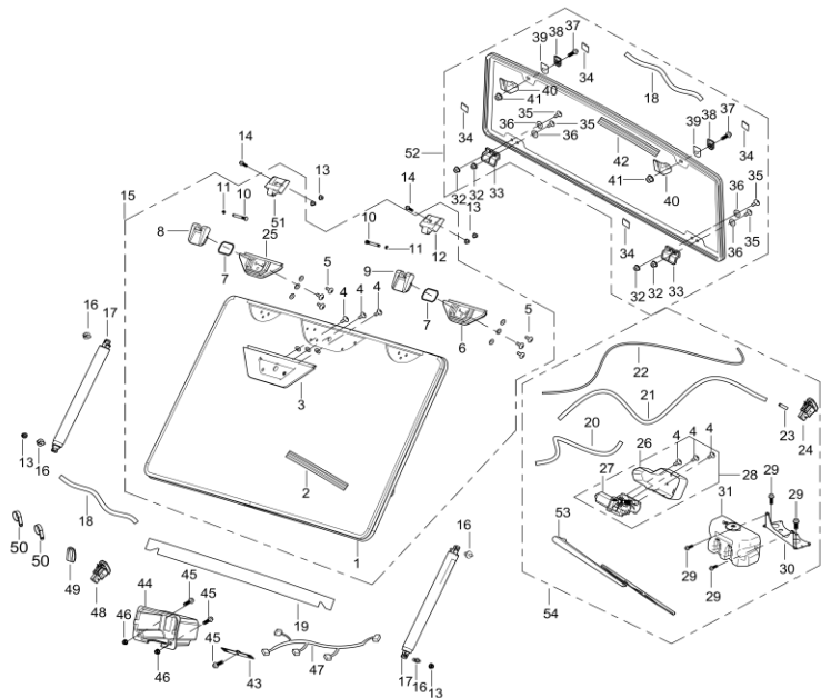
DIAGRAM 2026 FRONT AND REAR WINDOW(OPTIONAL) F27 Part 2
