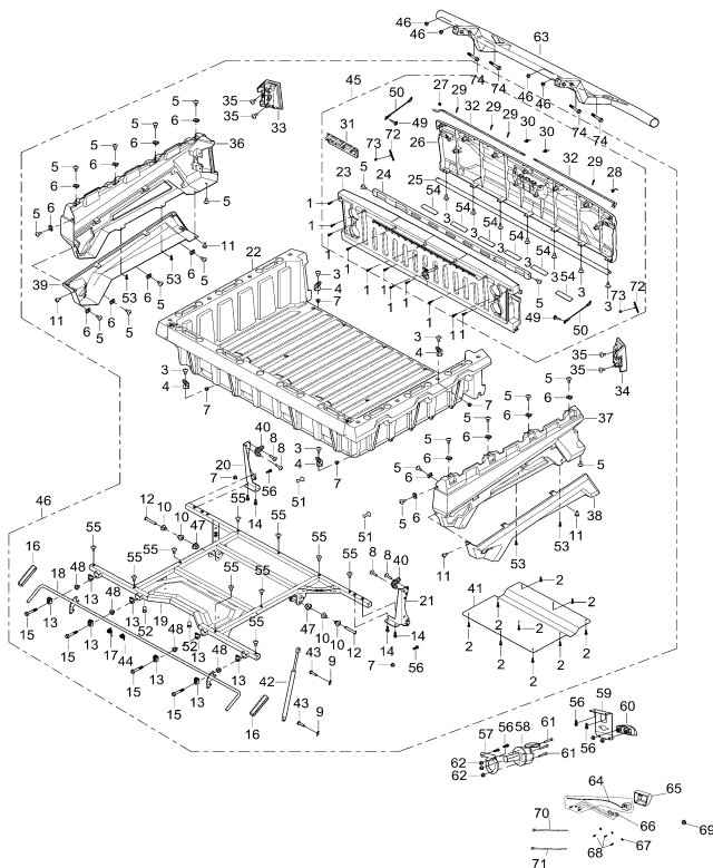
DIAGRAM 2026 CARGO BOX F21-Part 3
