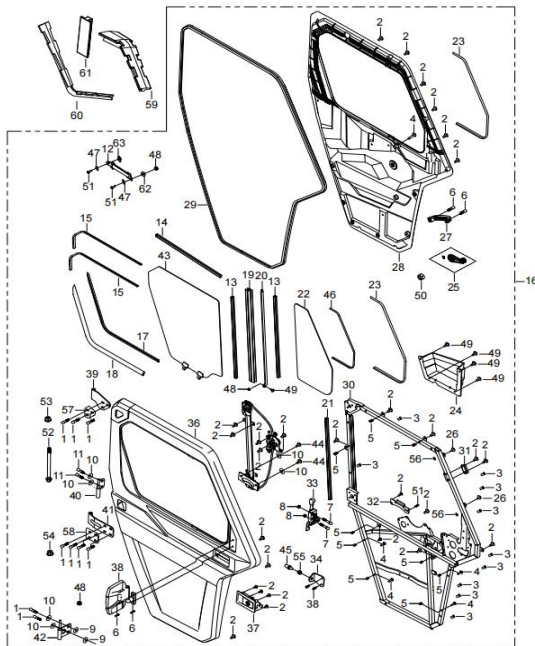
DIAGRAM 2026 FRONT DOOR PASSENGER SIDE (TWO DOOR) F25-Part 1
