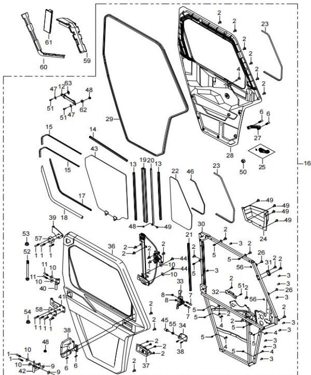
DIAGRAM 2026 FRONT DOOR PASSENGER SIDE (TWO DOOR) F25-Part 1
