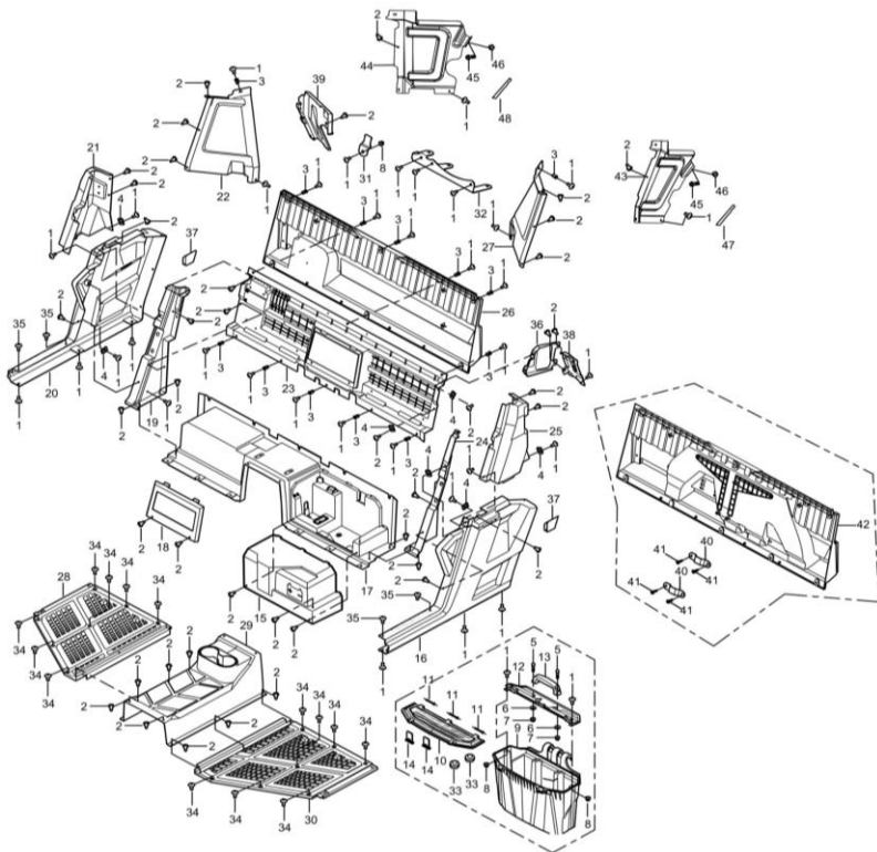
DIAGRAM 2026 REAR MUDGUARD AND FOOTBOARD (TWO DOOR)F19
