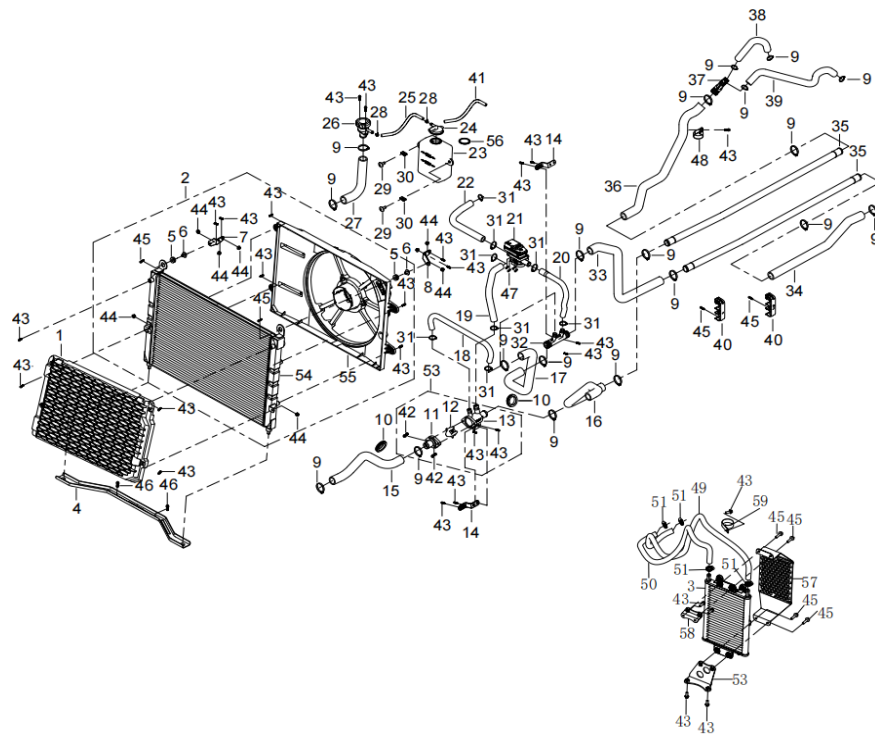
DIAGRAM 2026 COOLING SYSTEM(2 Door) F07-Part1
