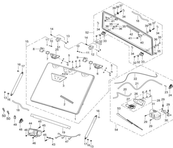
DIAGRAM 2026 FRONT AND REAR WINDOW(OPTIONAL) F27 Part 1
