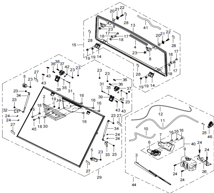
DIAGRAM 2026 FRONT AND REAR WINDOW(OPTIONAL) F27 Part 2
