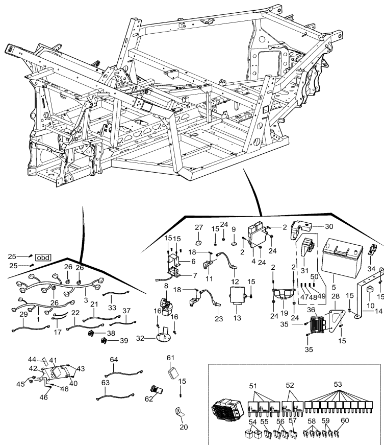
DIAGRAM 2026 ELECTRICAL COMPONENTS F22-Part 2
