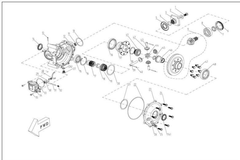
DIAGRAM 2026 Front Differential Assy SYSTEM
