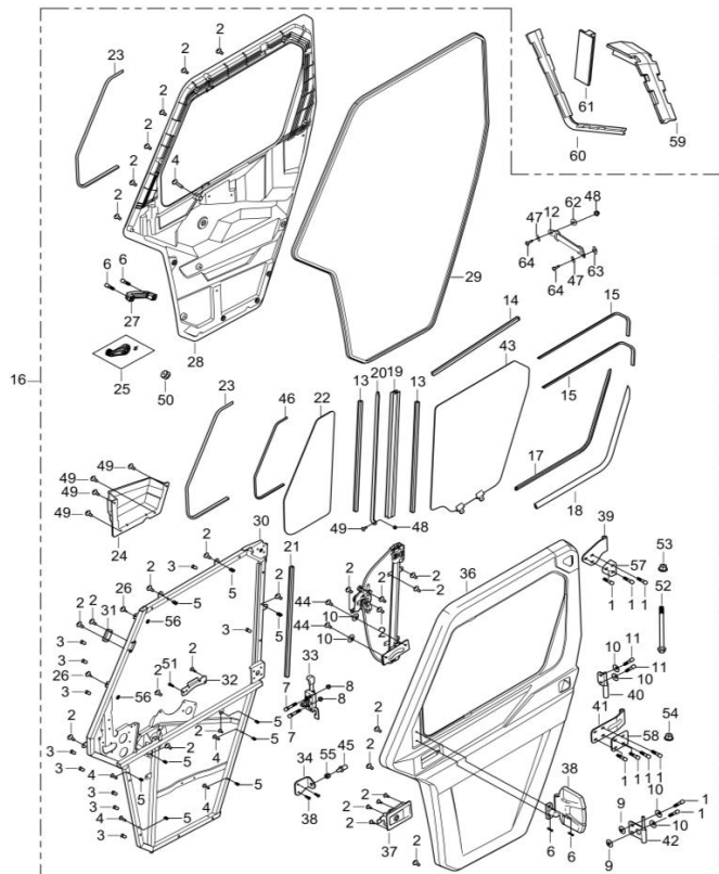
DIAGRAM 2026 FRONT DOOR DRIVER SIDE (TWO DOOR) F24-Part 3
