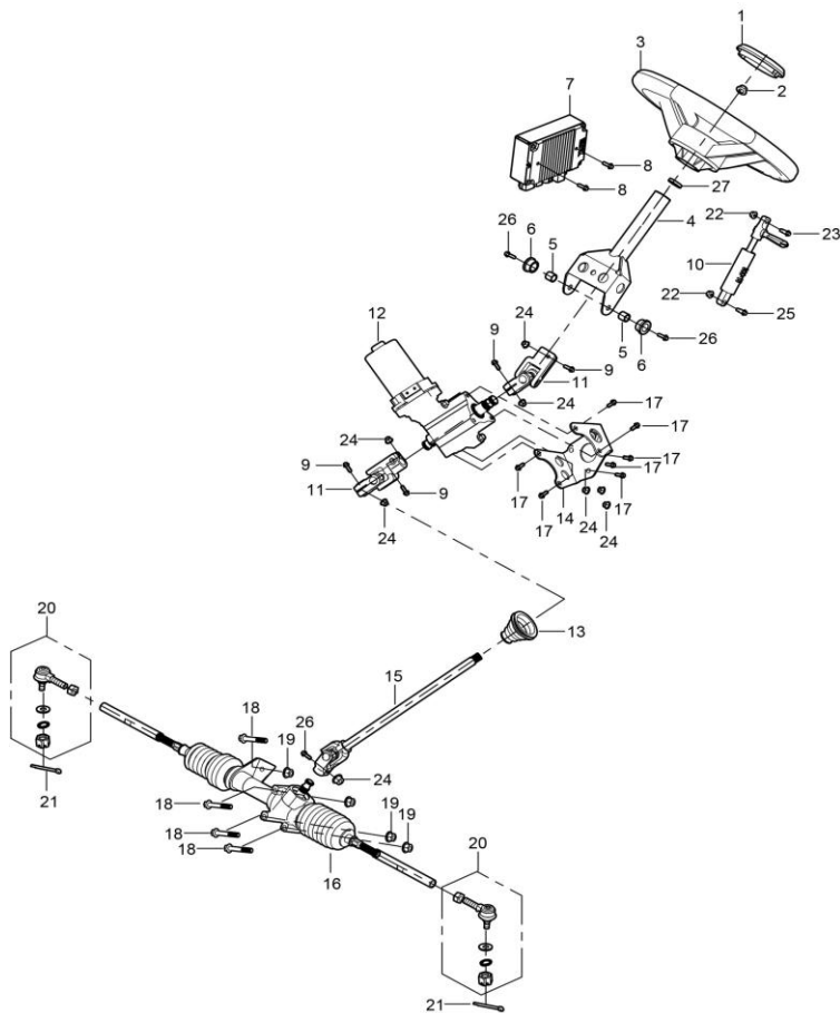
DIAGRAM 2026 STEERING SYSTEM(WITH EPS) F06
