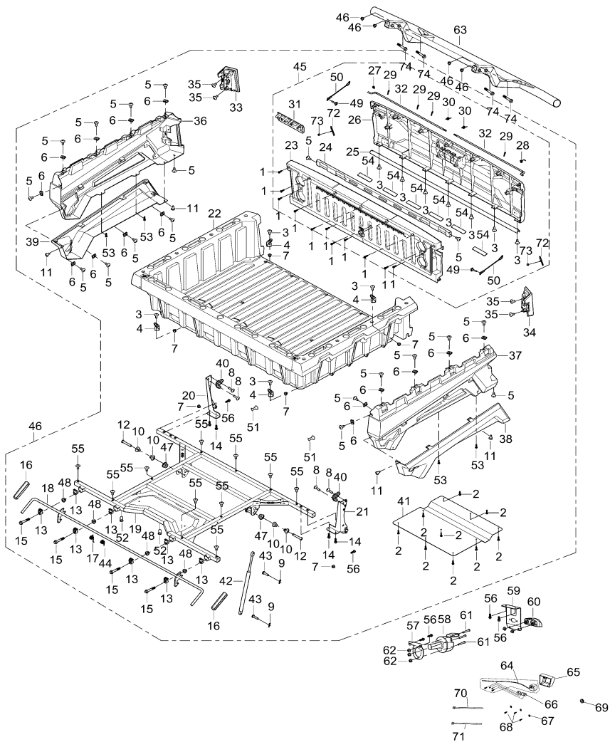
DIAGRAM 2026 CARGO BOX F21-Part 2
