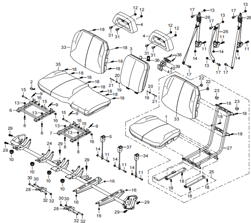
DIAGRAM 2026 SEATS (TWO DOOR) F14
