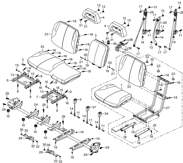
DIAGRAM 2026 SEATS (TWO DOOR) F14
