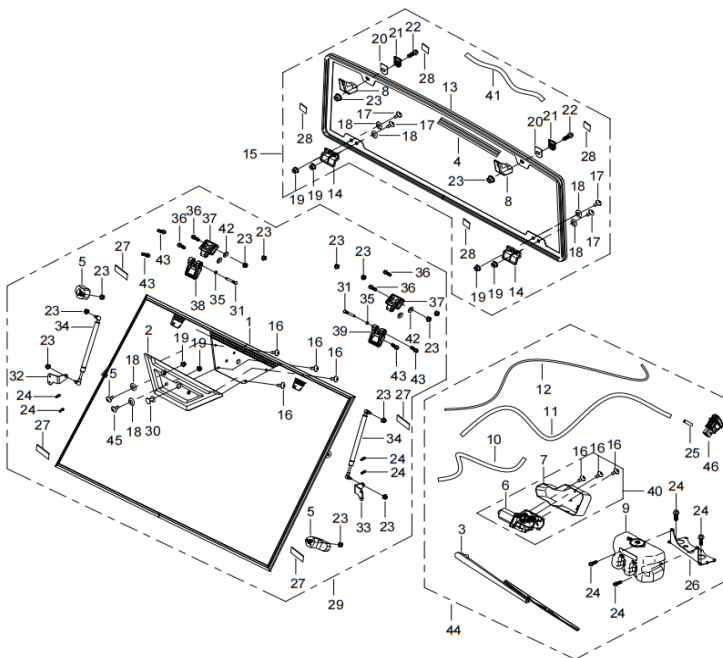
DIAGRAM 2026 FRONT AND REAR WINDOW(OPTIONAL) F27 Part 1
