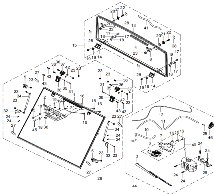
DIAGRAM 2026 FRONT AND REAR WINDOW(OPTIONAL) F27 Part 2
