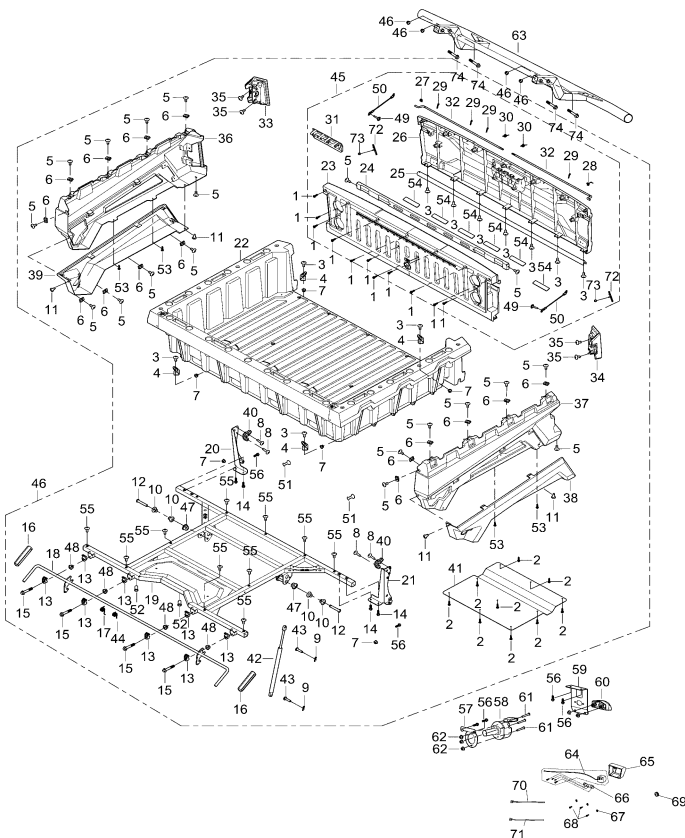
DIAGRAM 2026 CARGO BOX F21-Part 1
