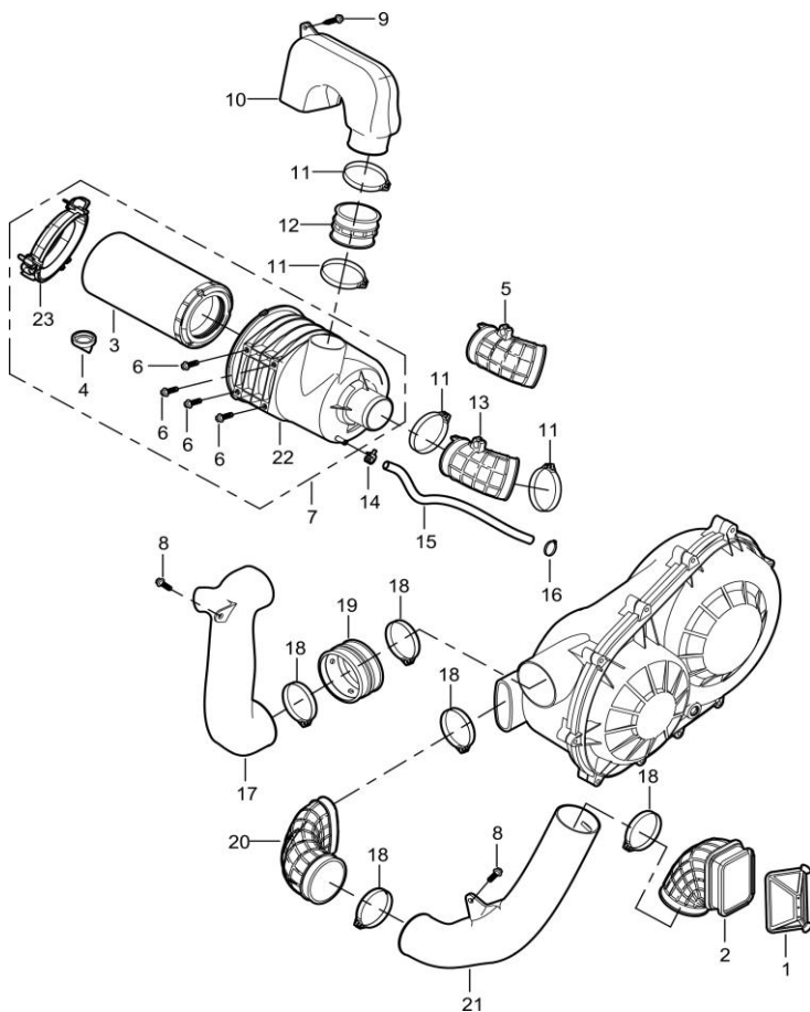
DIAGRAM 2026 AIR FILTER & CVT INLET&OUTLET SYSTEM F09
