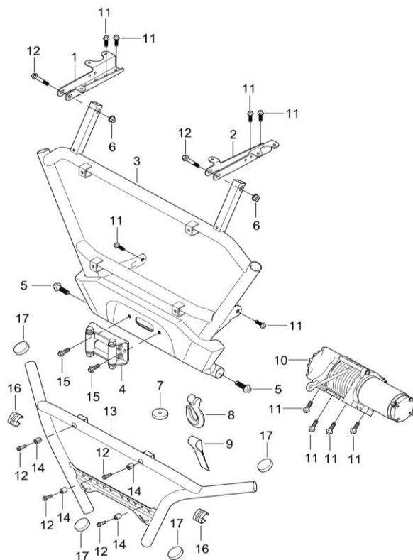
DIAGRAM 2026 FRONT WINCH AND BUMPER F20
