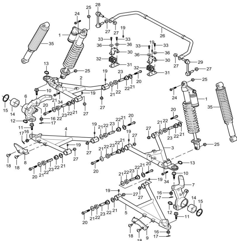
DIAGRAM 2026 FRONT SUSPENSION SYSTEM F01
