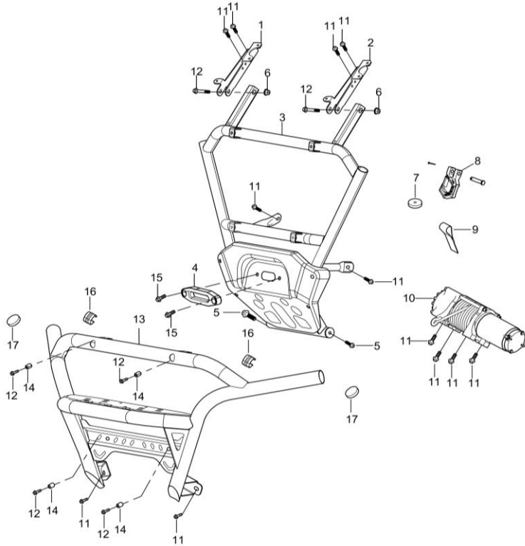
DIAGRAM 2026 FRONT WINCH AND BUMPER (2026YEAR)选配 F20
