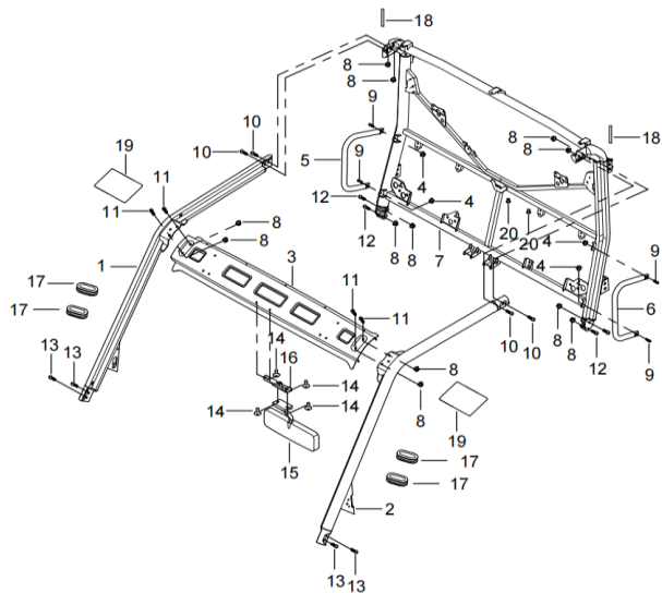
DIAGRAM 2026 ROLL BAR (TWO DOOR) F11
